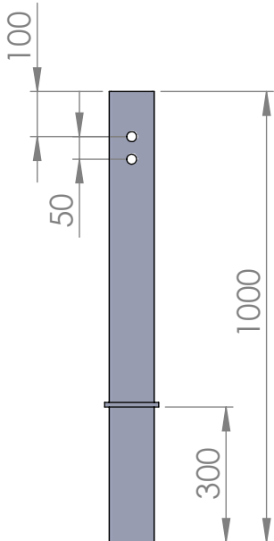
T-12651 - FOURREAU 100X100 LG 1000 U 16
