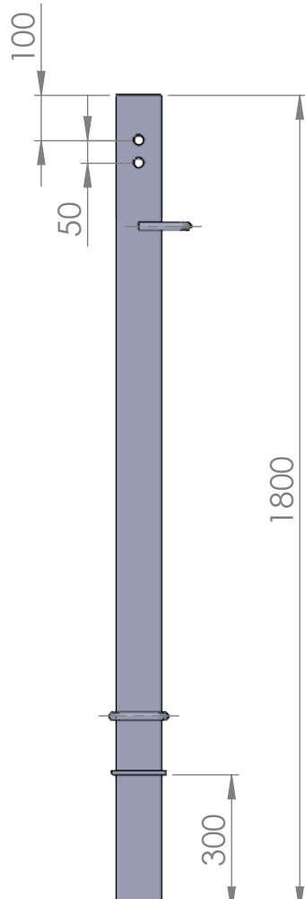
T-12671 - FOURREAU 100X100 LG 1800 U 16
