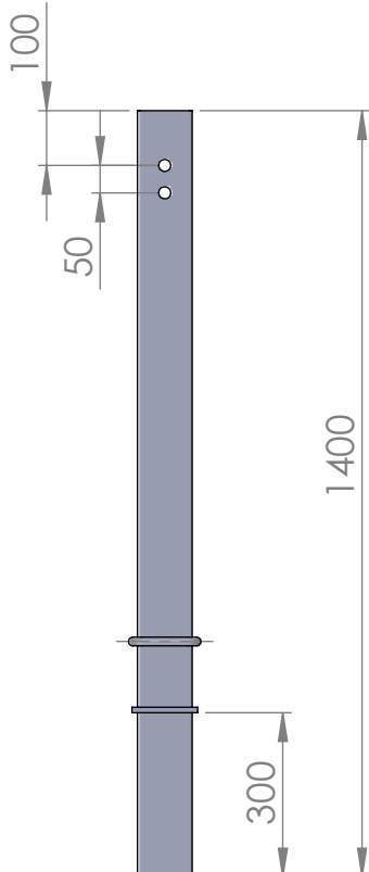
T-12661 - FOURREAU 100X100 LG 1400 U 16
