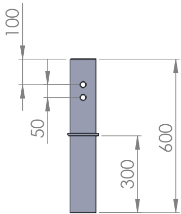
T-12641 - FOURREAU 100X100 LG 600 U 16
